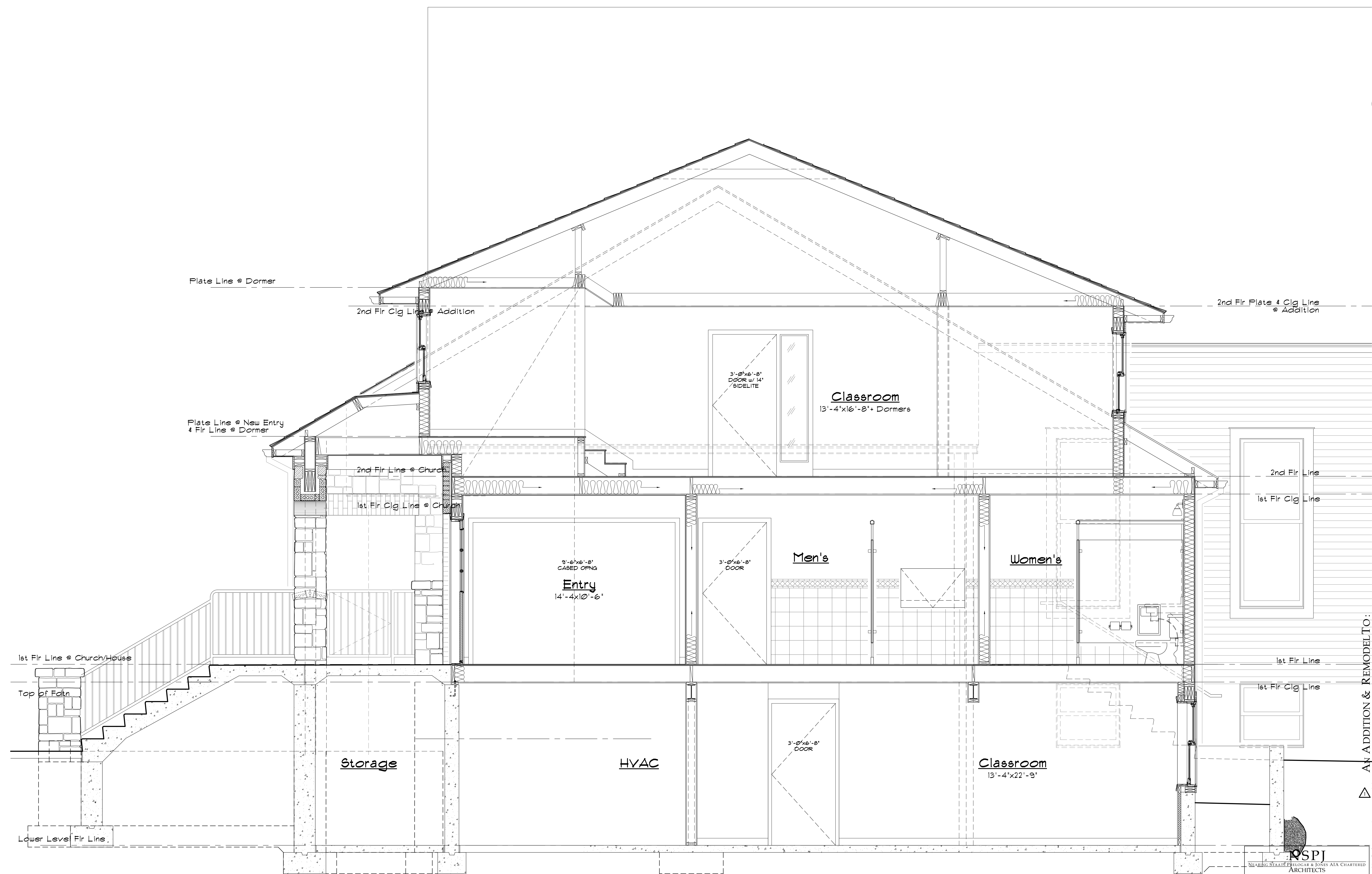
Bldg Section - Looking West 1/2" = 1'-0" (A/1)
