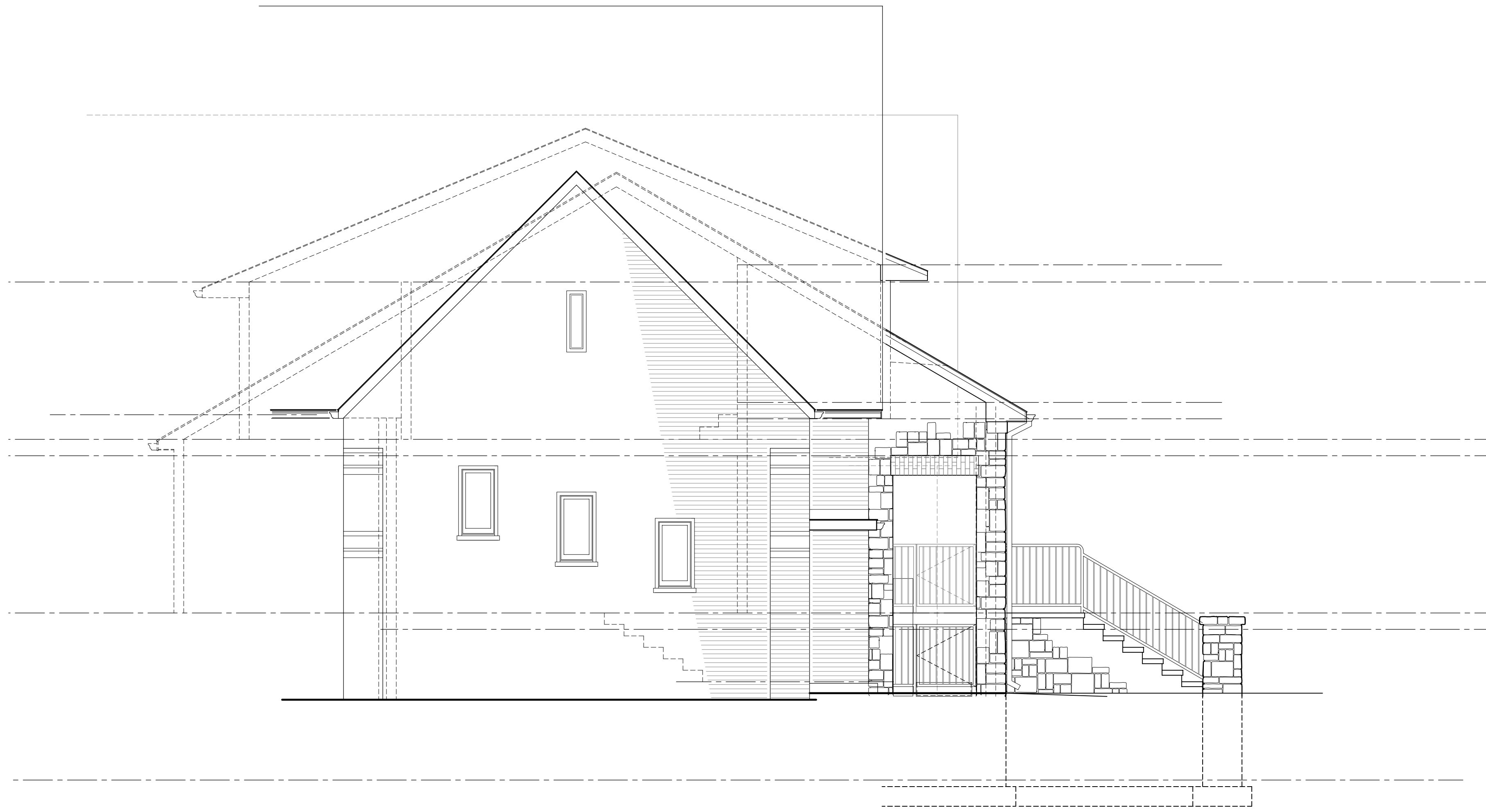
Partial West Elevation \frac{1}{4}'' = 1'-0''
