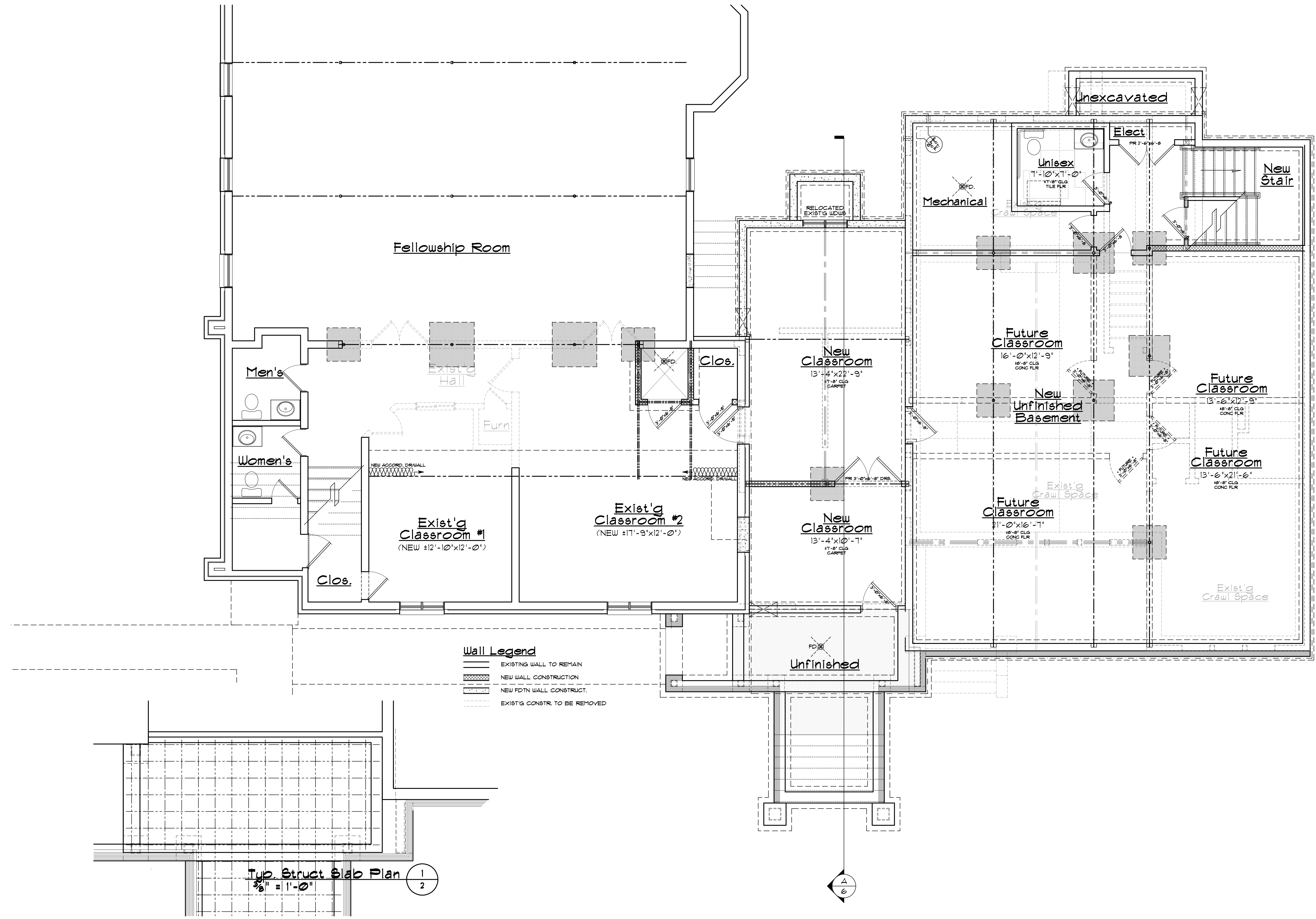
Partial Lower Level Plan 1/4" = 1'-0" Approx. Addition Area = 341 sqft. NORTH
